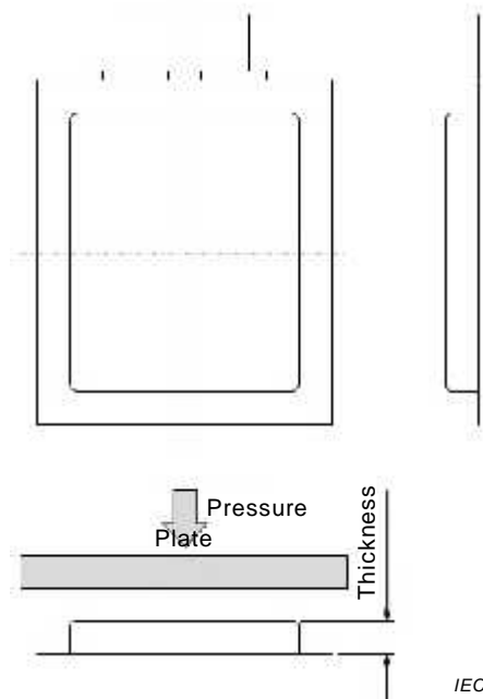
Figure A.1 – Thickness measuring method
