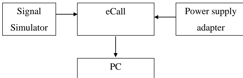
Figure 2: Diagram of test stand
