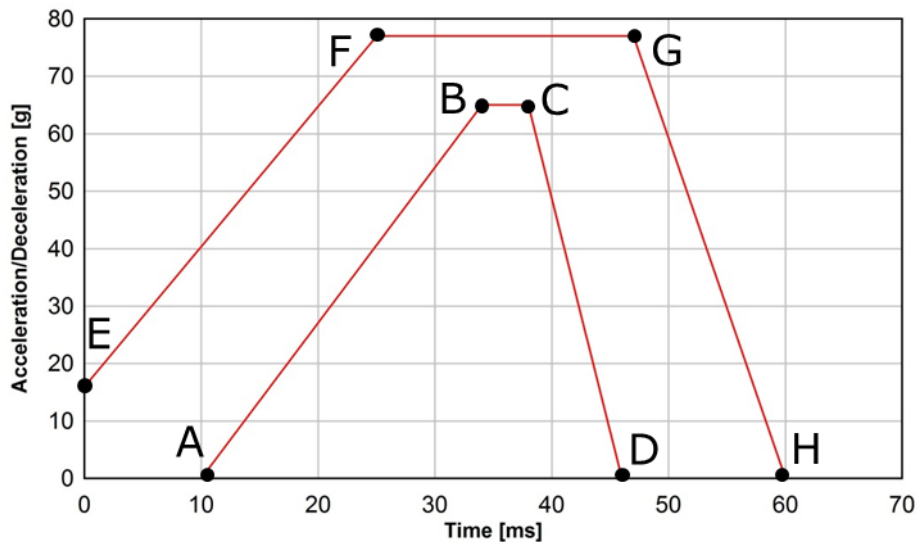
Figure 1: Minimum and maximum curve of the test pulse (pulse corridor)
